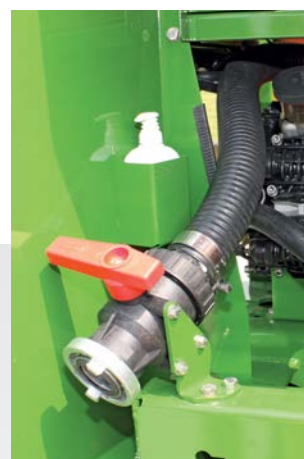
Bowser filling (C coupling or Camlok coupling)
